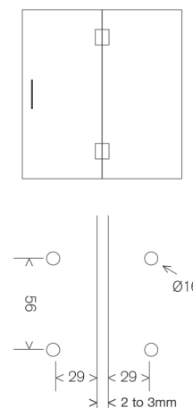
MF2-BF Glass to Glass BiFold Hinge
