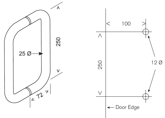
MD250 Delta Handle
