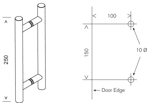
GTFR150 and GTFS150 Fineline Handle
