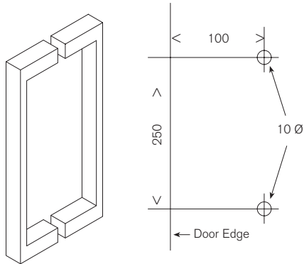
GT-Q250 Rectangular Pull Handle
